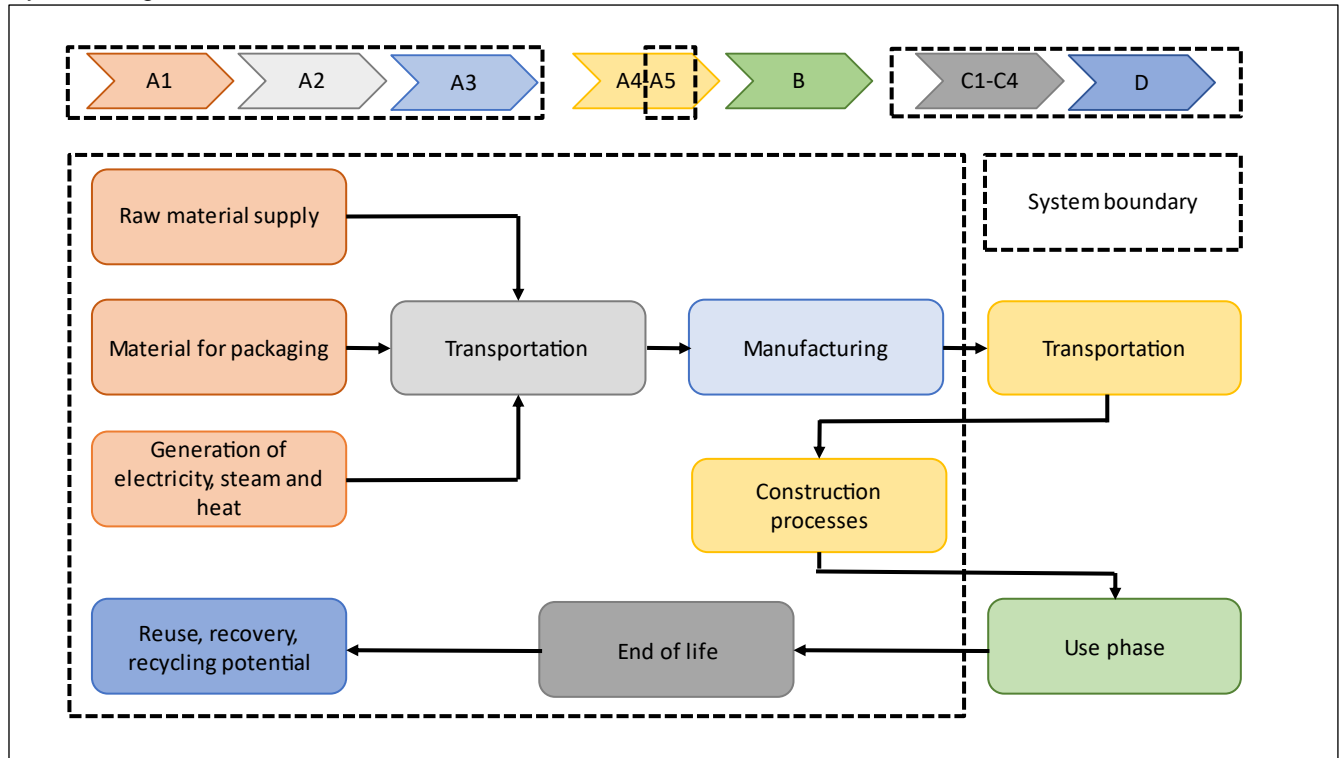
Figure 1 System boundary of the LCA study conducted on FATRAFOL 807 - HETEROGENEOUS WATERPROOFING MEMBRANE
